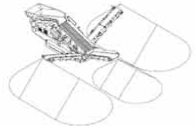
Fines Belt Discharge Height 12'- 6" (3.8m) Midsize Belt Discharge Height 13' - 0" (3.8M) Oversize Belt Discharge Height 9' - 6" (2.9m)
